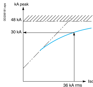
Current limiting.
