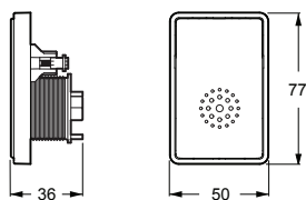
IHC CONTROL® Alarm lyd giver Intern LK FUGA
