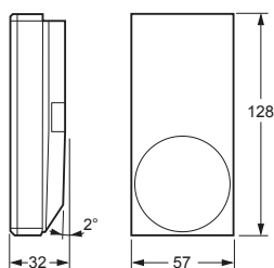
IHC CONTROL® Alarm PIR 12 V / PDM-IXA12
