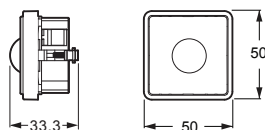
IHC CONTROL® PIR 24 V LK FUGA, 90 grader
