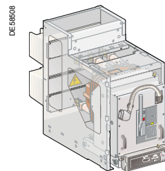
Withdrawable
